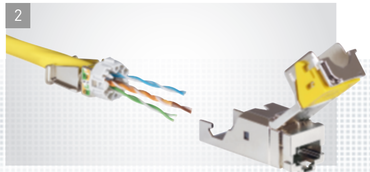
2 Pass the cable through the back of the wire housing
